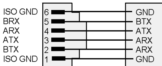
RS485-MODBUS - FULL DUPLEX
