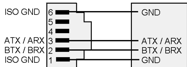
RS485-MODBUS - HALF DUPLEX
